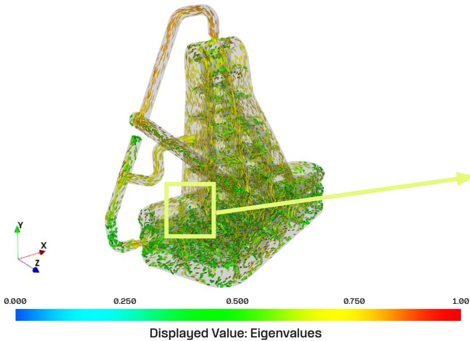
Fiber Orientation Results Load Bracket
